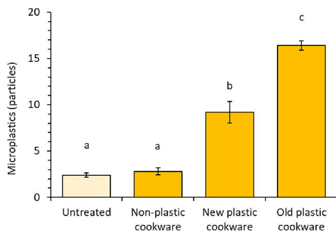
Fig. 2. Microplastic contamination of food simulant before (light yellow) and after (dark yellow) cooking using different cookware ( n = 5 per treatment). Data presented as mean with standard error bars. Different letters denote significant differences between treatments (Kruskal–Wallis with pairwise Wilcoxon test, P < 0.05 ).
